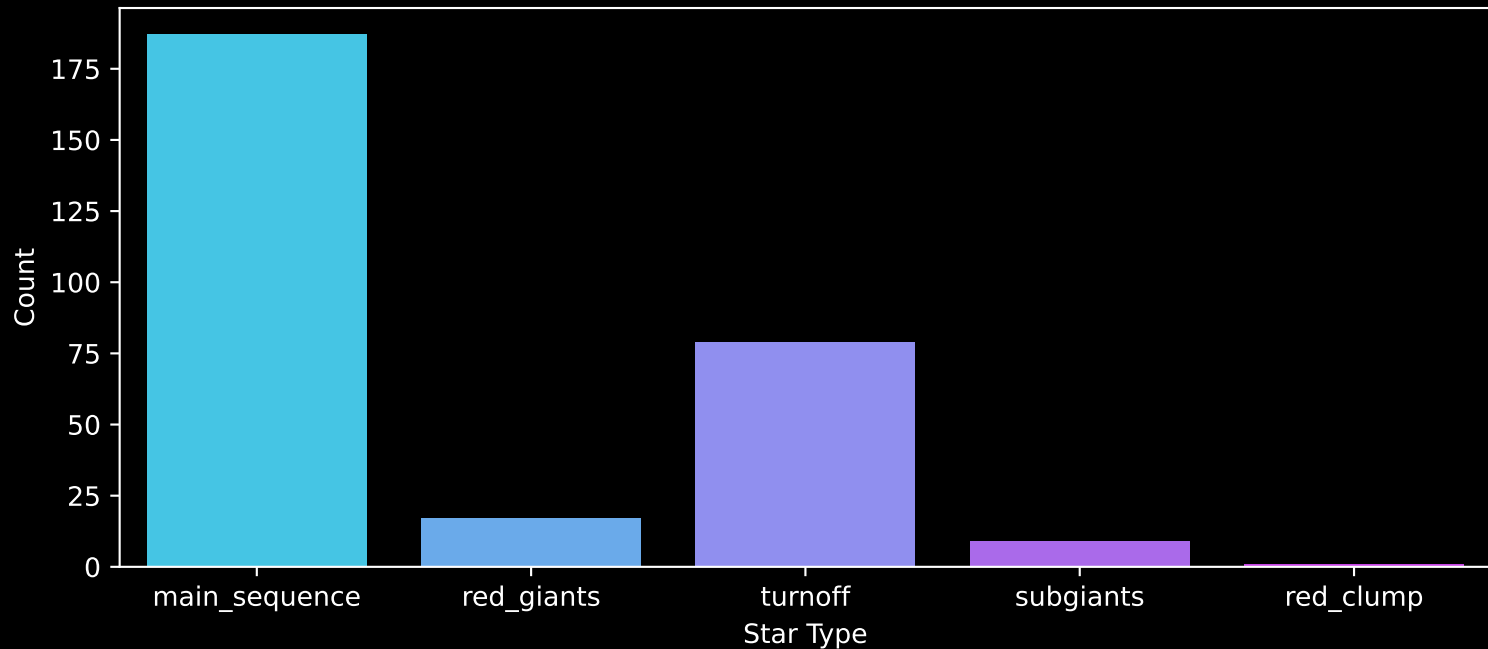
GALAH DR4 Field: [7003] Count plot of Star Type
