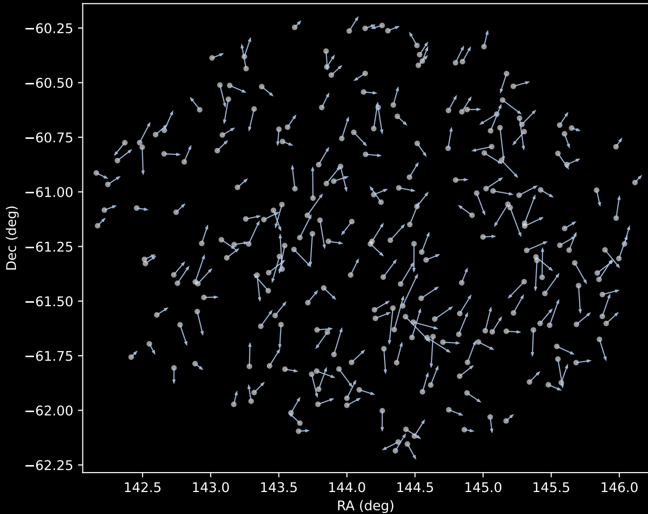
GALAH DR4 Cluster 1 Proper Motion Vectors (n=243)
