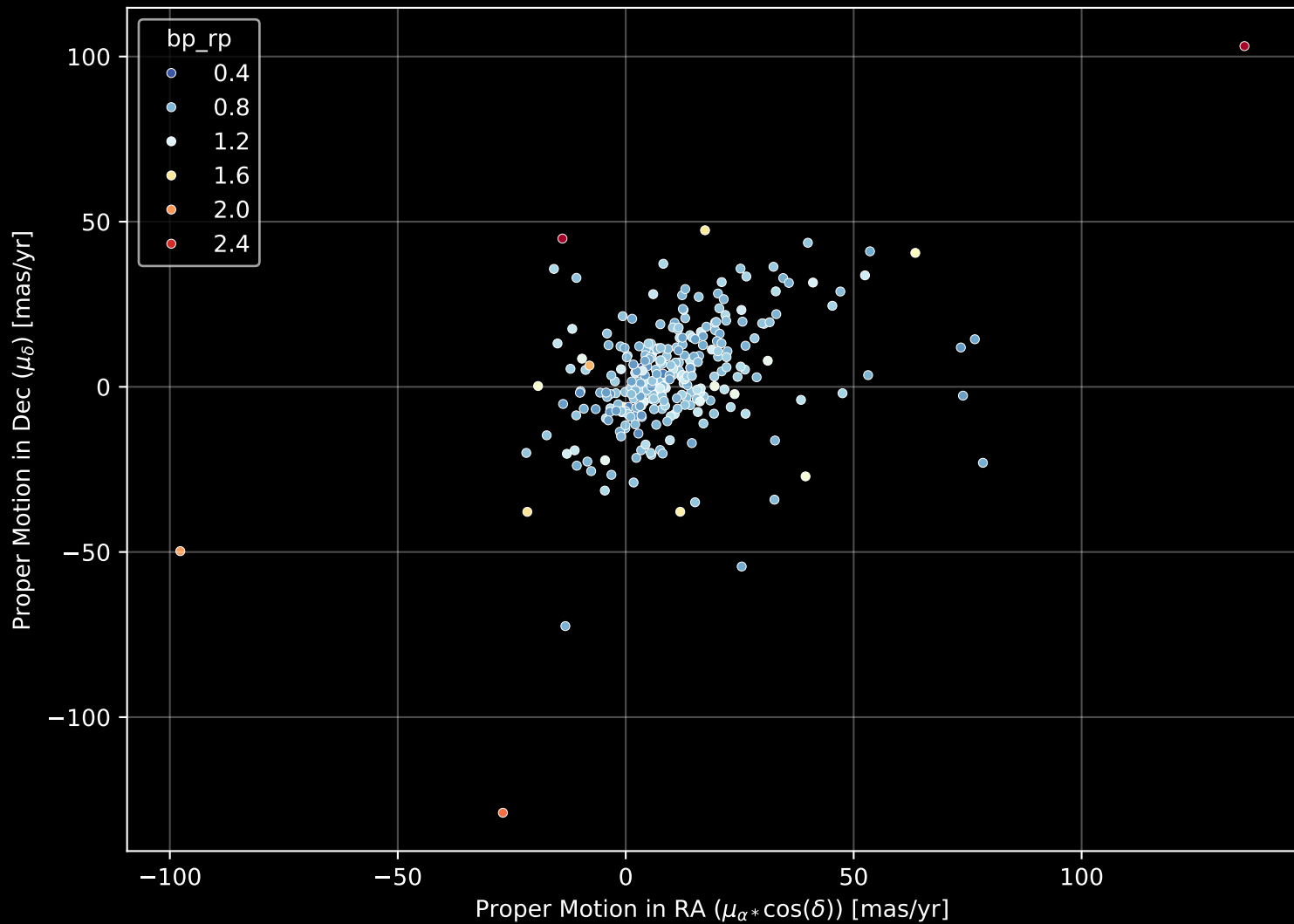
GALAH DR4 Field: [7003] Proper Motion Diagram (n= 293)
