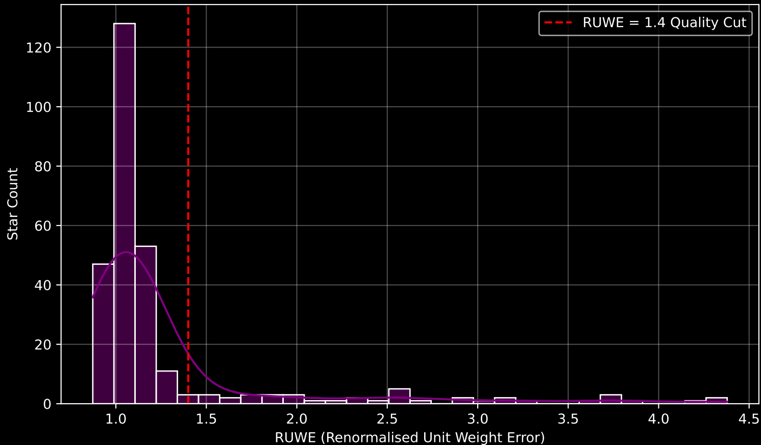
GALAH DR4 Field [7003] RUWE Distribution (n= 281)
