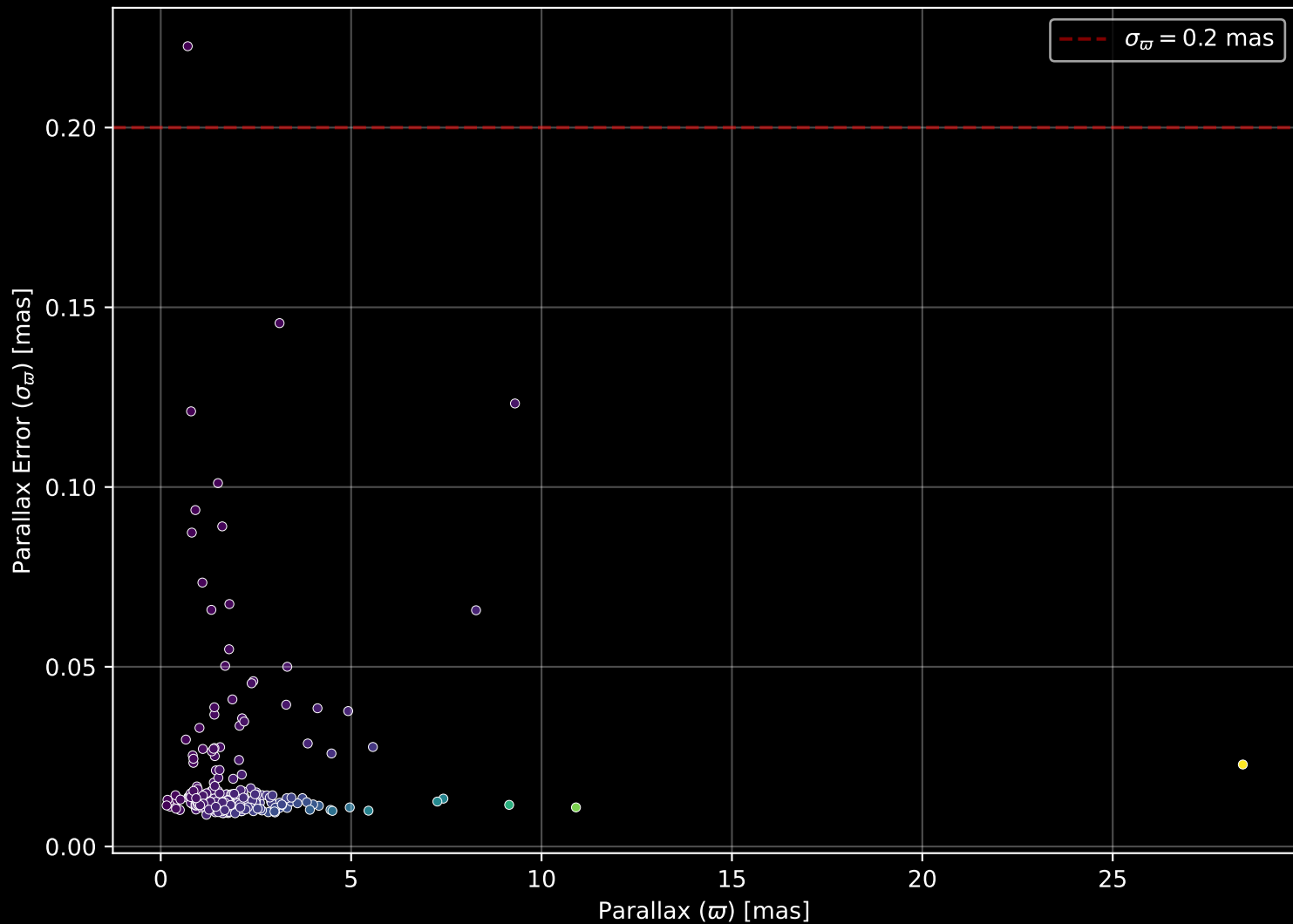
GALAH DR4 Field: [7003] Parallax Quality (n= 293)
